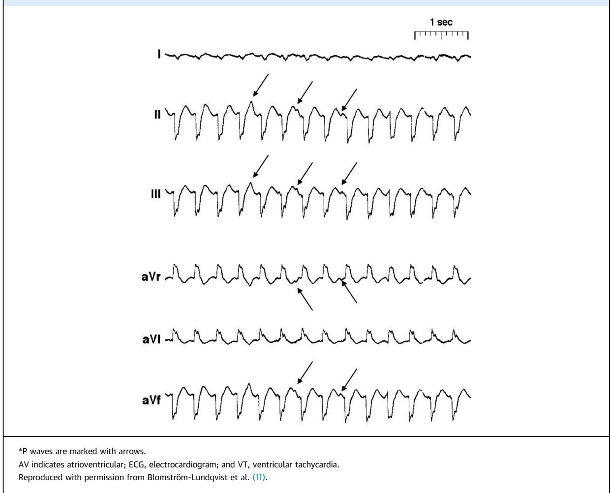
FIGURE 1 ECG Showing AV Dissociation During VT in a Patient With a Wide-QRS Complex Tachycardia
